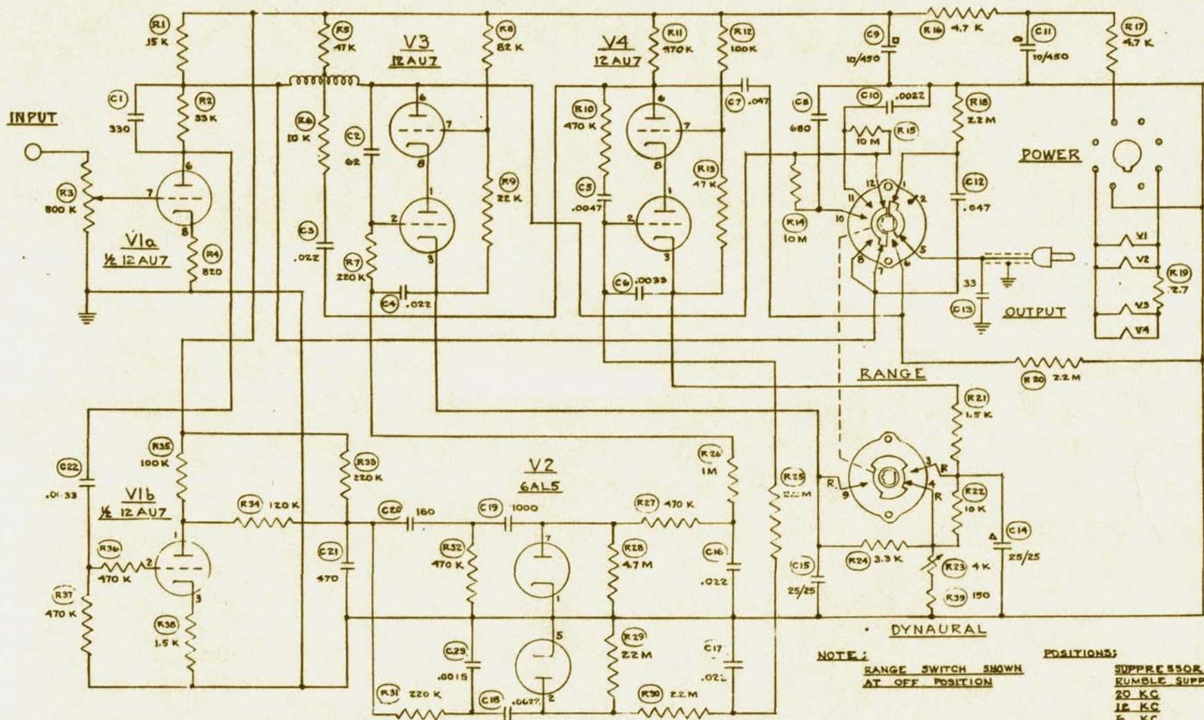
114-A DYNABURAL NOISE SUPPRESSOR CIRCUIT DIAGRAM
