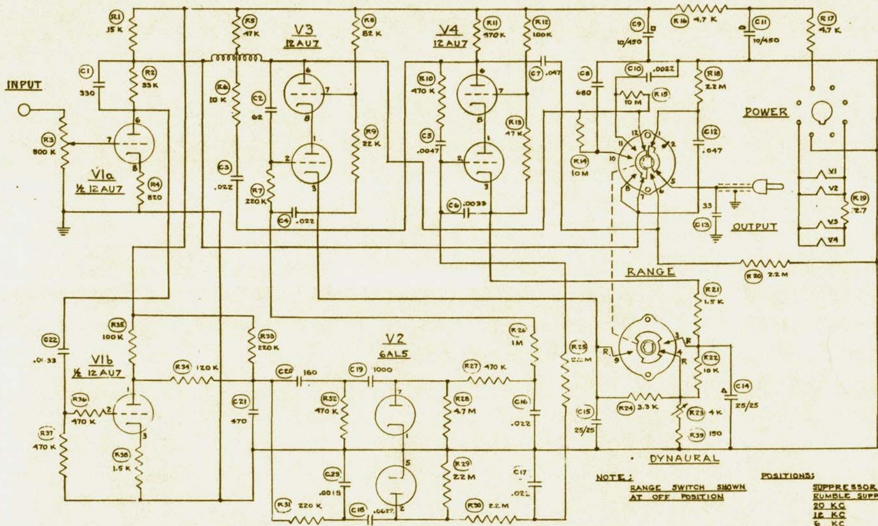
114-A DYNAURAL NOISE SUPPRESSOR CIRCUIT DIAGRAM
