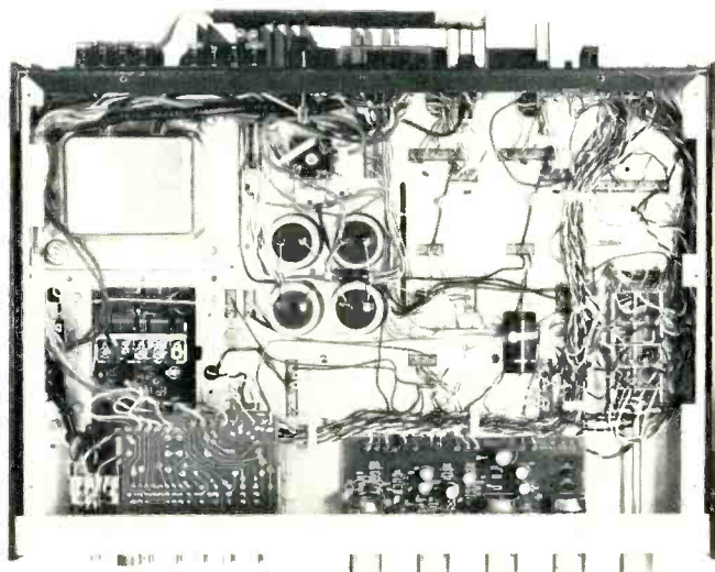
Fig. 2—Internal view of the receiver.
