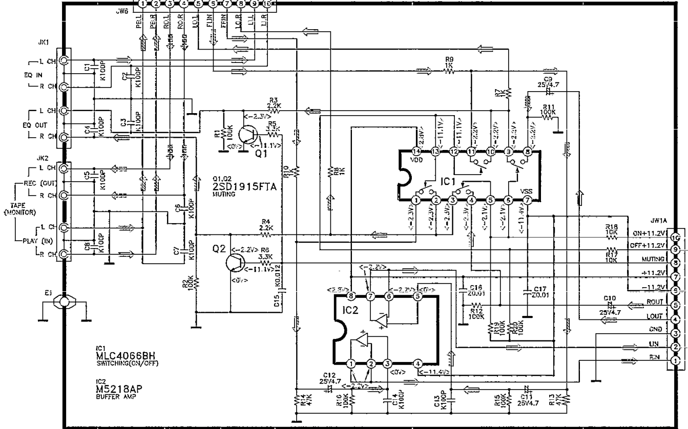
A IN/OUTPUT TERMINAL/BUFFER AMP CIRCUIT
